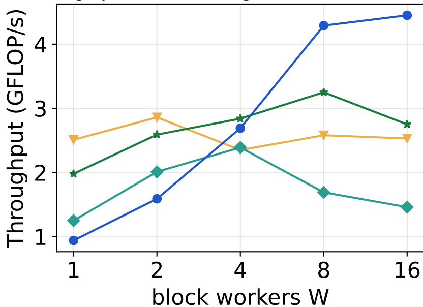
Throughput vs block-grid W (1024×1024)
